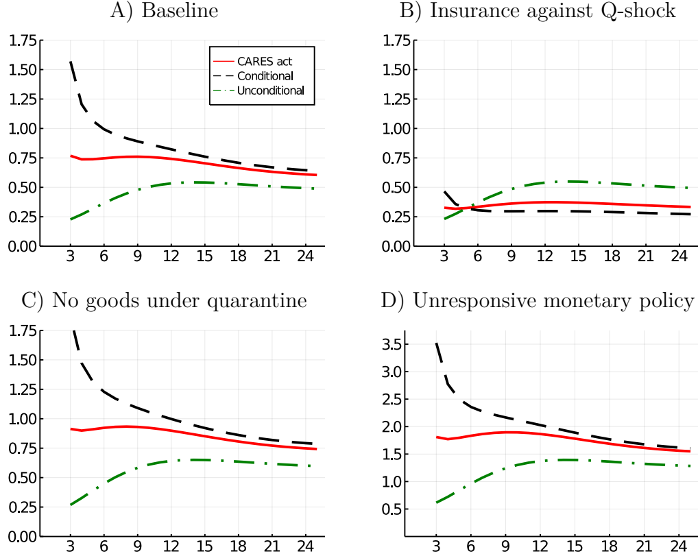
Figure 5: Cumulative transfer multipliers. Notes: Cumulative multiplier computed as \sum_{j=1}^k y_i / \sum_{j=1}^k t_i , where y_i is the deviation of output from baseline, t_i is the transfer payment (both measured in percentage points of steady-state output), and k is the time since announcement in period 1 (February 2020), measured along the horizontal axis. We report multipliers from period k = 3 onward, since transfers are zero or very small in the first two periods.
