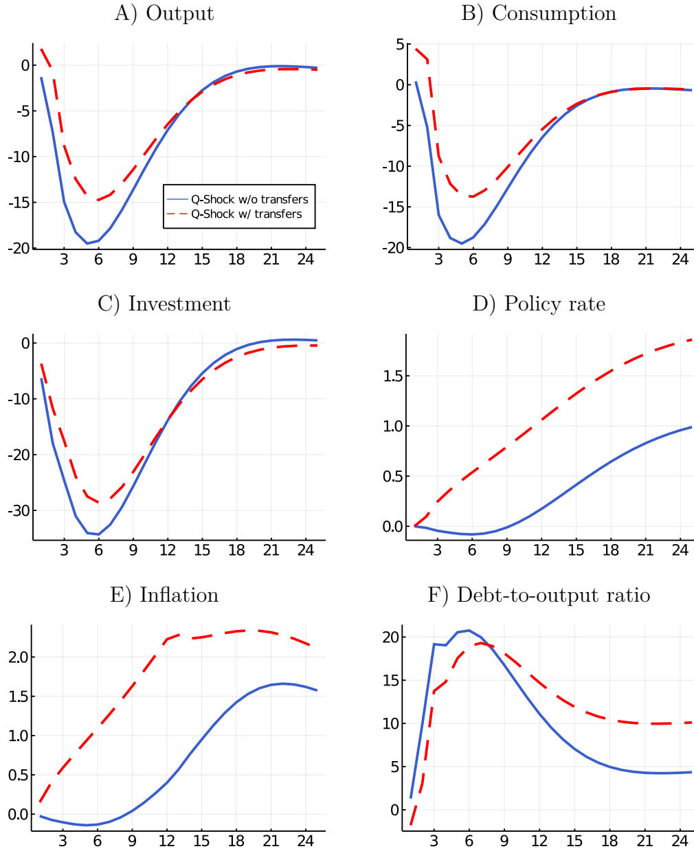
Figure 4: Dynamic adjustment to Q-shock with and without fiscal transfers. Notes: Red dashed line shows response w/ transfers, blue solid line w/o; see Figure 2 for details on the Q-shock. Inflation is computed using the actual price index P_t^F rather than the ideal price index P_t . Y-axis: Percentage deviation from steady state, annualized percentage points in case of (y-o-y) inflation and interest rate. X-axis: Months.
