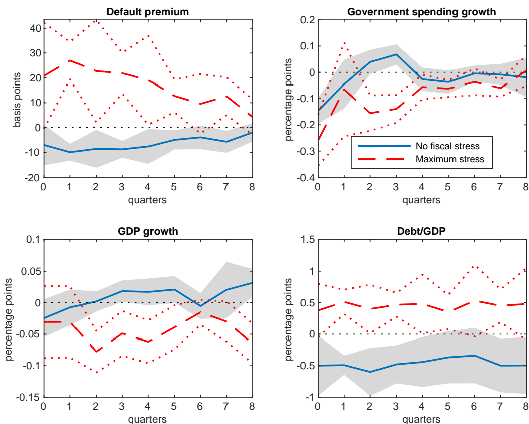
Figure 4: Dynamic adjustment to fiscal shock (reduction of government consumption by 1 percentage point annualized) in times of no fiscal stress (solid line) and in times of maximum stress (dashed line). Notes: horizontal axis measures quarters, vertical axis measures deviation from pre-shock path in percentages and basis points (default premium). Shaded areas and dotted lines indicate 90 percent confidence bounds. Results based on Oxford Economics forecast sample where debt data is available.
