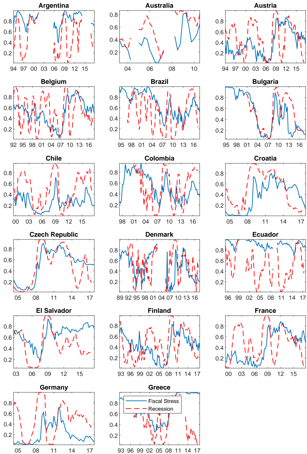
Figure B.2: Values of empirical CDF (Country group-specific) for lagged default premia and smoothed output gaps.
