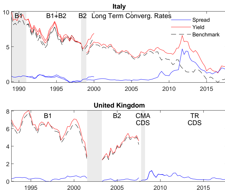
Figure A.1: Construction of sovereign yield spread: Italy and United Kingdom.
